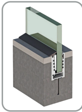
OS-AL-06 60 (H) x 34 (W) Counseled Profile
