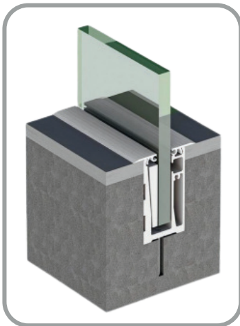
OS-AL-05 115 (H) x 60 (W) Counseled Profile
